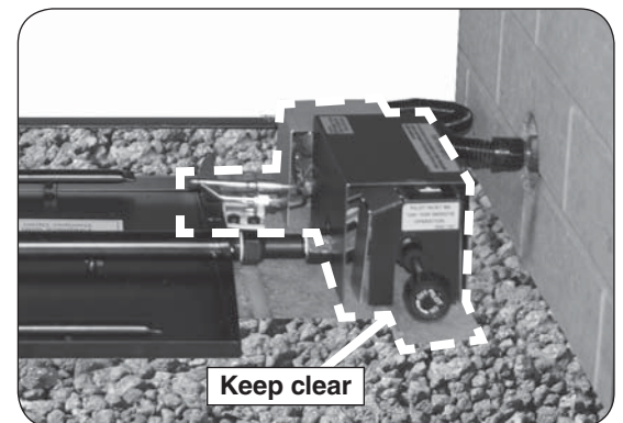
Fig. 19-3 Proper lava media placement
