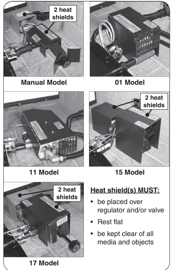
Fig. 19-1 Place heat shield(s)
