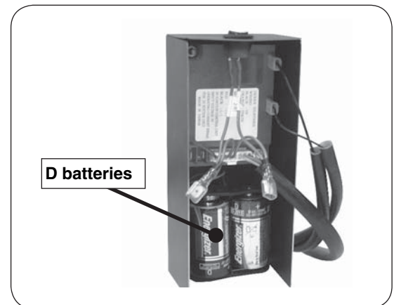
Fig. 23-3 Switch box batteries (01 models)
