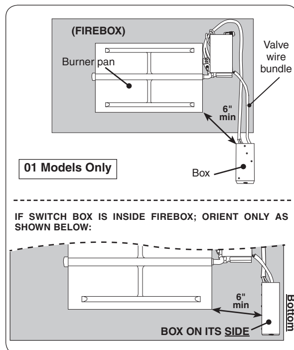
Fig. 17-3 Switch box placement (if applicable)
