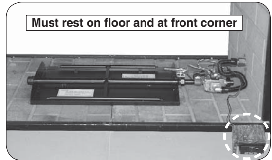
Fig. 18-2 Place heat shield (if applicable)
